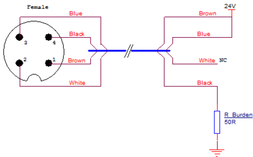
Figure 3 Dewpoint measurement.
