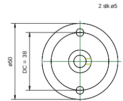
Adjustable flange AISI 316
